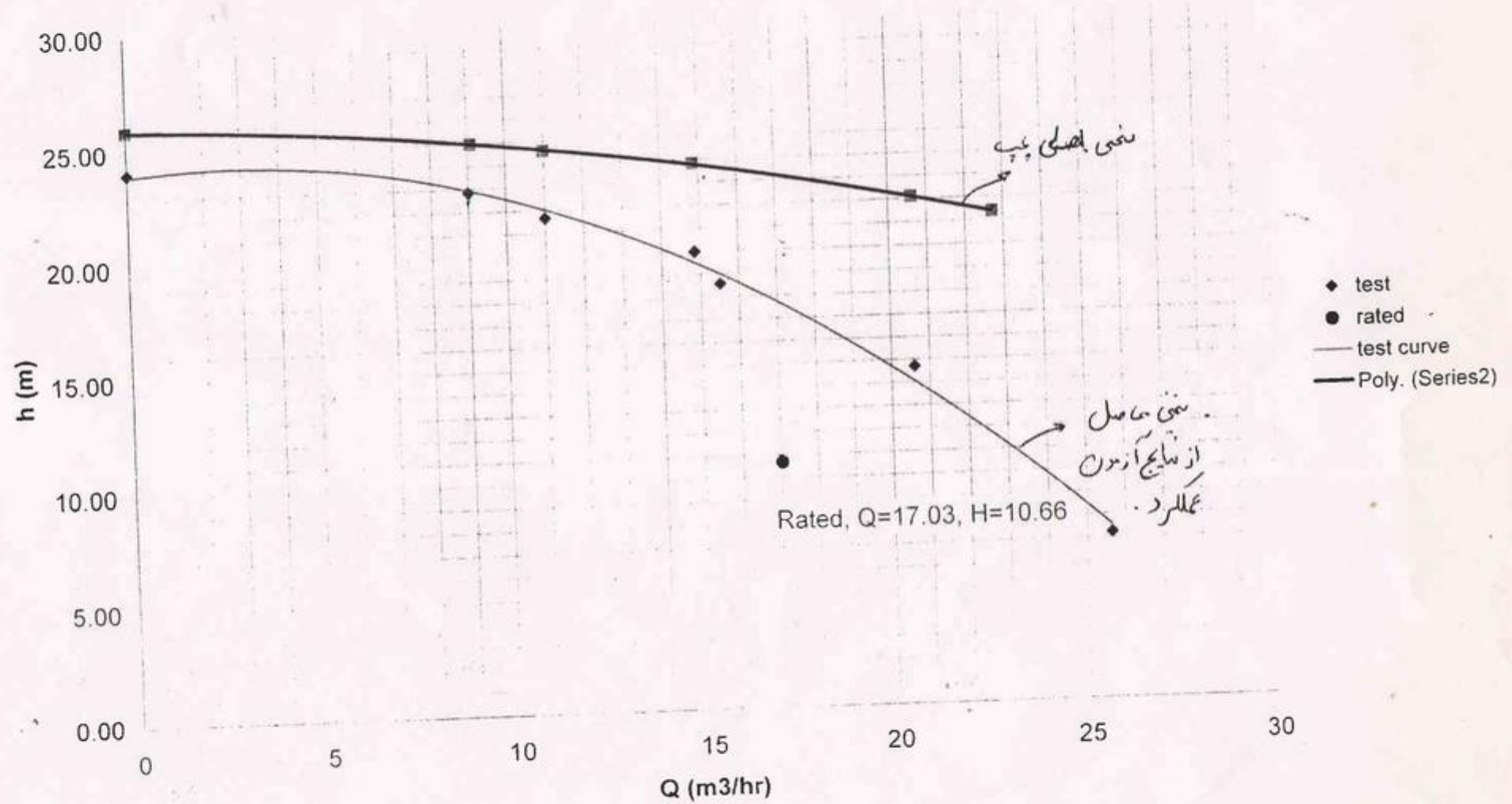
Performance test curve (mission pump type 1* 1 1/2)
